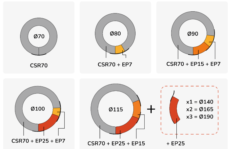
Example of diameter configurations using modular extension parts.
